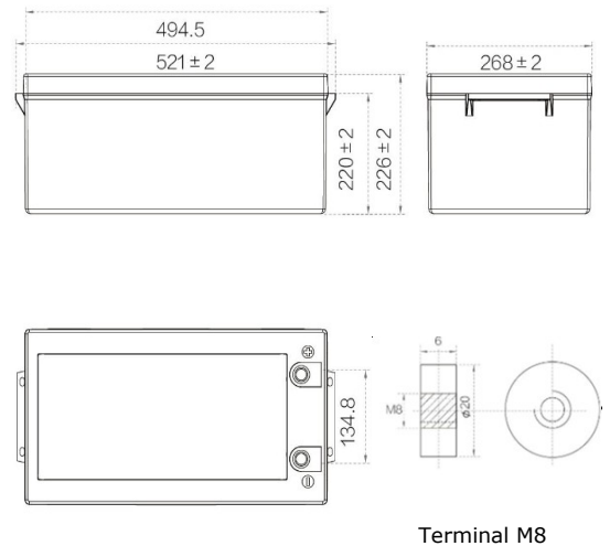
Terminal M8
