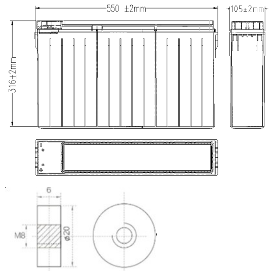
Terminal M8
